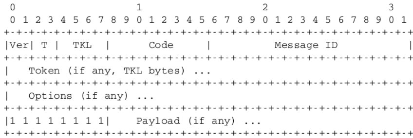
Figura 2.4: Header COAP
